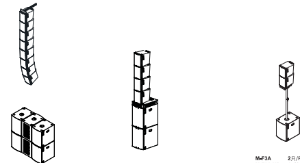
M-F3A BF 1面/PC M-F3A 8面/PCS S12 PRO 6面/PCS 带有M-F3A BF吊架的M-F3A线性阵列 M-F3A line array hanging system with M-F3A BF M-F3A 4面/PCS M-F3A SFI 1面/PC S12 PRO 2面/PCS M-F3A通过M-F3A SFI堆叠安装到M-F3A S12 PRO上面 Ground stacking of M-F3A and M-F3A S12 PRO with M-F3A SFI M-F3A 2面/PCS M-F3A UB 1面/PC SPS 20 1面/PC S12 PRO 1面/PC M-F3A通过M-F3A UB、SPS 20堆叠安装到M-F3A S12 PRO上面 Pole mounting of M-F3A and M-F3A S12 PRO with M-F3A UB and SPS 20
